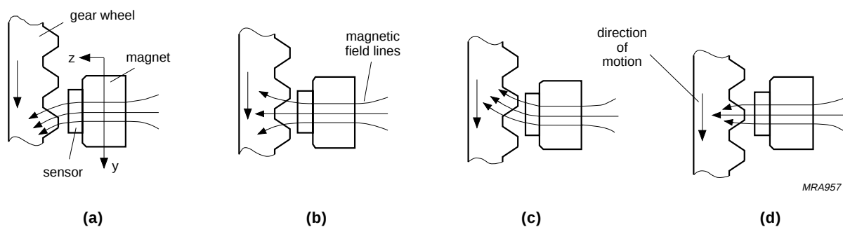
Fig.3 Functional principle.
